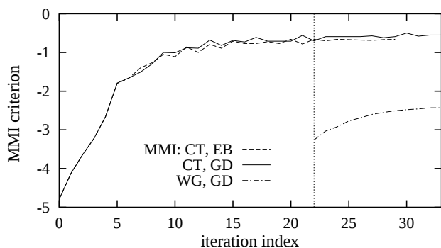
Figure 1: MMI criterion for the male speakers of the SieTill training corpus for corrective training (CT) and the use of word graphs (WG).
