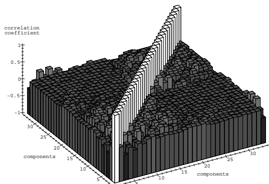
Figure 2: Correlations between the components of the acoustic vector: filter-bank coefficients ( top ) and cepstrum coefficients ( bottom ).
