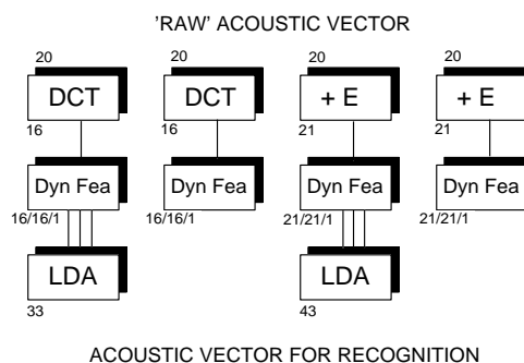
Figure 1: Four different configurations of the acoustic front-end based on cepstral decorrelation (DCT), inclusion of frame energy (+E), inclusion of spectral dynamic features (DynFea) and linear discriminant analysis (LDA).
