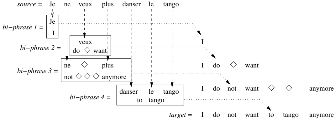
Figure 2: Combining bi-phrases to produce a translation.
