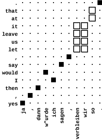
Figure 1: Example of a manually annotated alignment with sure (filled dots) and possible connections.
