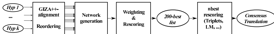
Figure 1: The system combination architecture.
